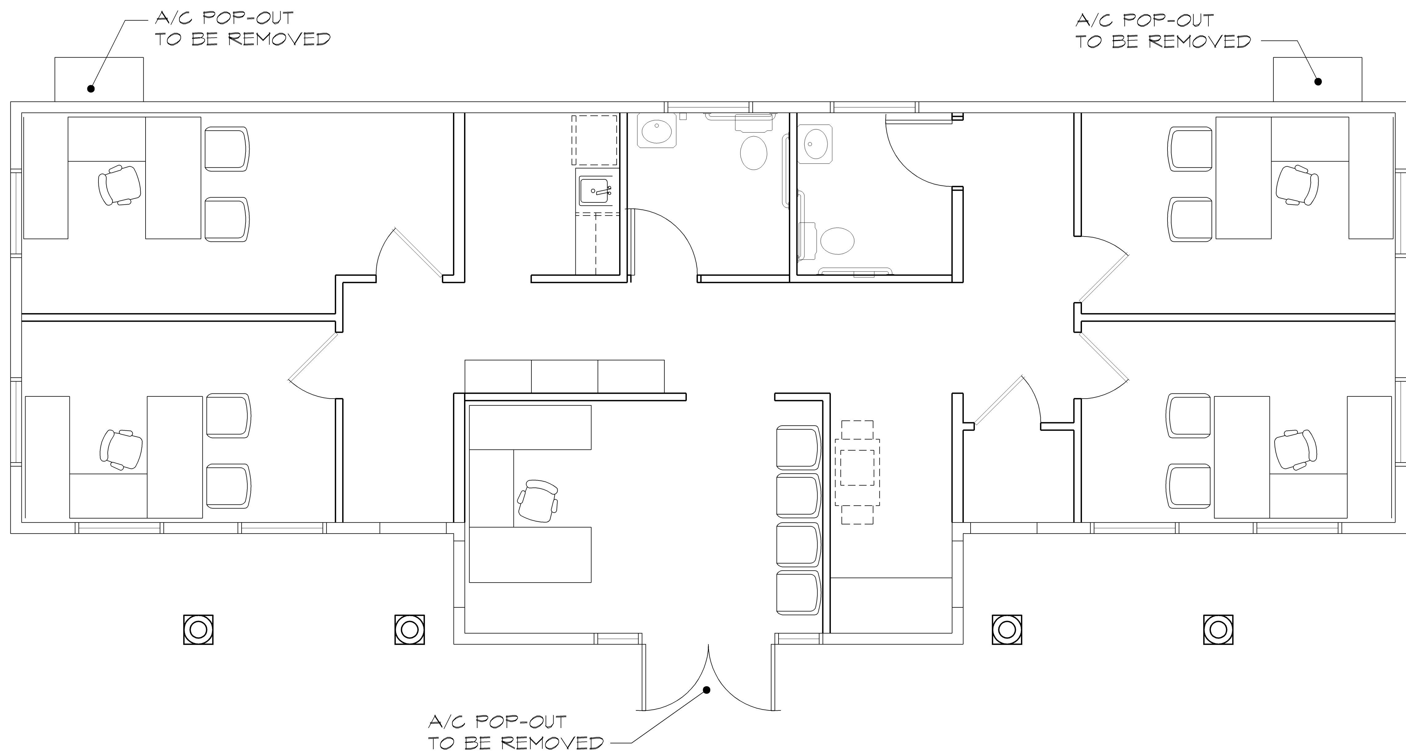
BUILDING "B" - FLOOR PLAN
